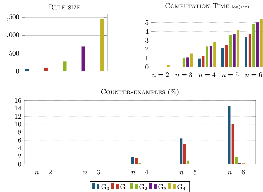
Fig. 9. Performance measures
