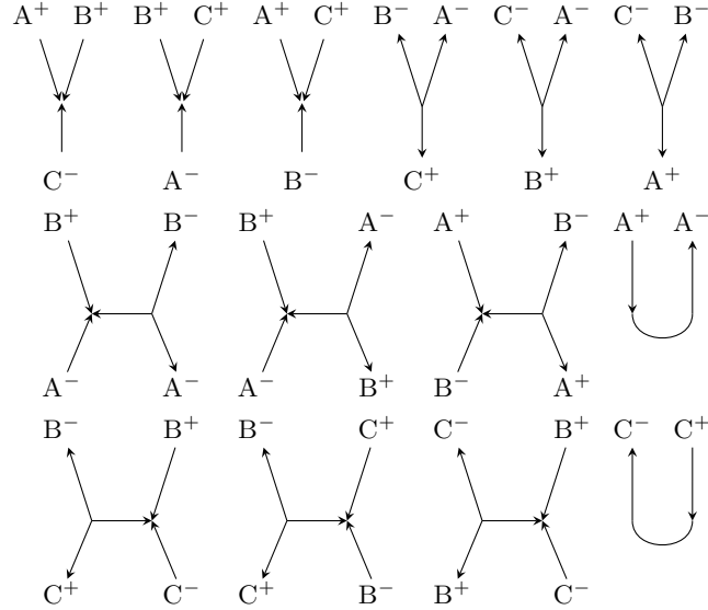
Fig. 5. Growth rules
